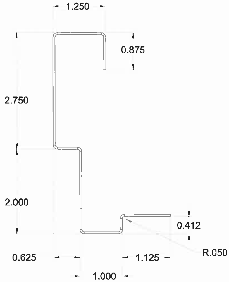
FRAME SECTION - 3 SIDES
